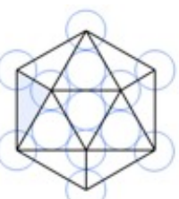
Icosahedron
